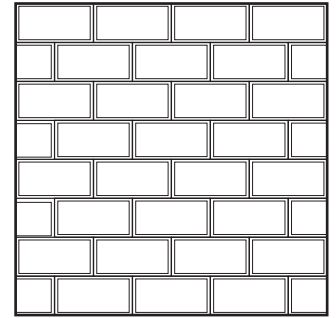
Running Bond 4" x 8" or 6" x 12"
