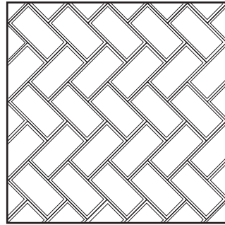
45° Herringbone* 4" x 8" or 6" x 12"
