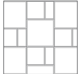
Installed Combination 4" x 8", 8" x 8" and 12" x 12"
